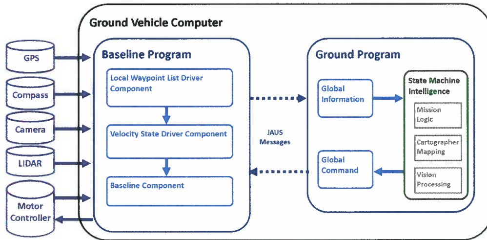
Figure 6. AUTOMATON Software Structure
