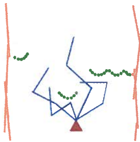
Figure 8. Conceptual example of beam search algorithm
